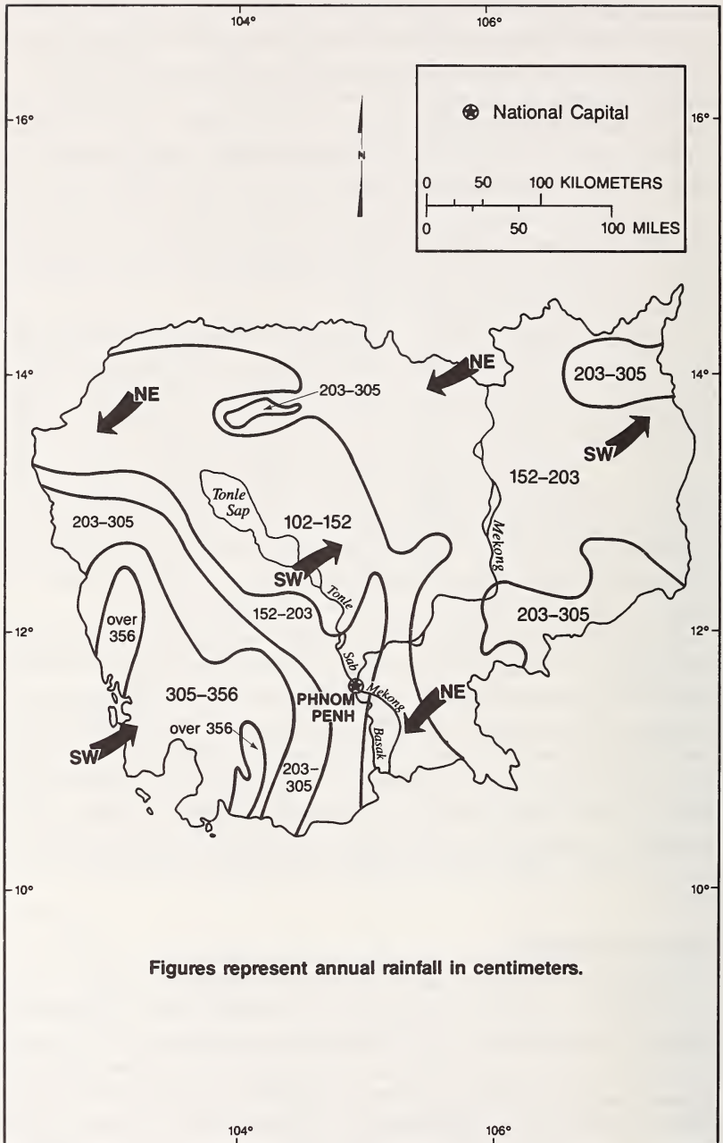
Figure 5. Annual Rainfall and Monsoon Airflow
